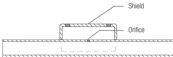
Cutaway view, standard configuration
